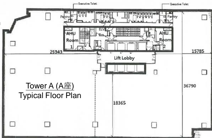
Floor Plan (for identification purpose only)
